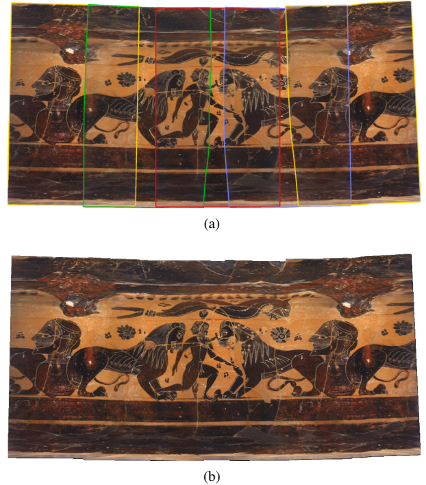
Figure 8: (a) Stitching of individual cylindrical unwrappings. Color boundaries indicate different views. (b) Multiresolution spline blending of the registered unwrappings [BA83].
